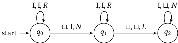
Figure 14.3: A machine computing f(x, y) = x + y
