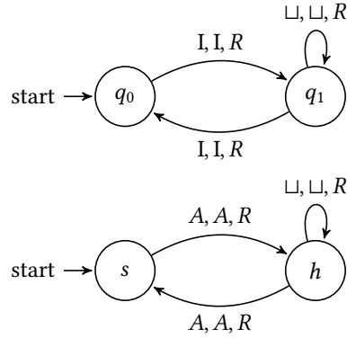
Figure 15.1: Variants of the Even machine
