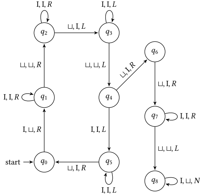
Figure 14.4: A machine computing f(x) = 2x
