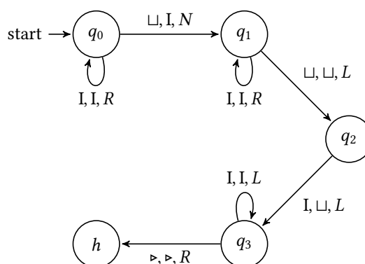
Figure 14.6: A disciplined addition machine
