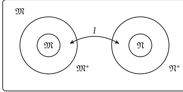
Figure 24.1: The structure \mathfrak{M} with the internal partial isomorphism.
