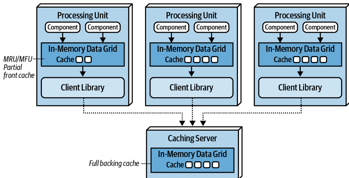
Figure 15-14. Near-cache topology
