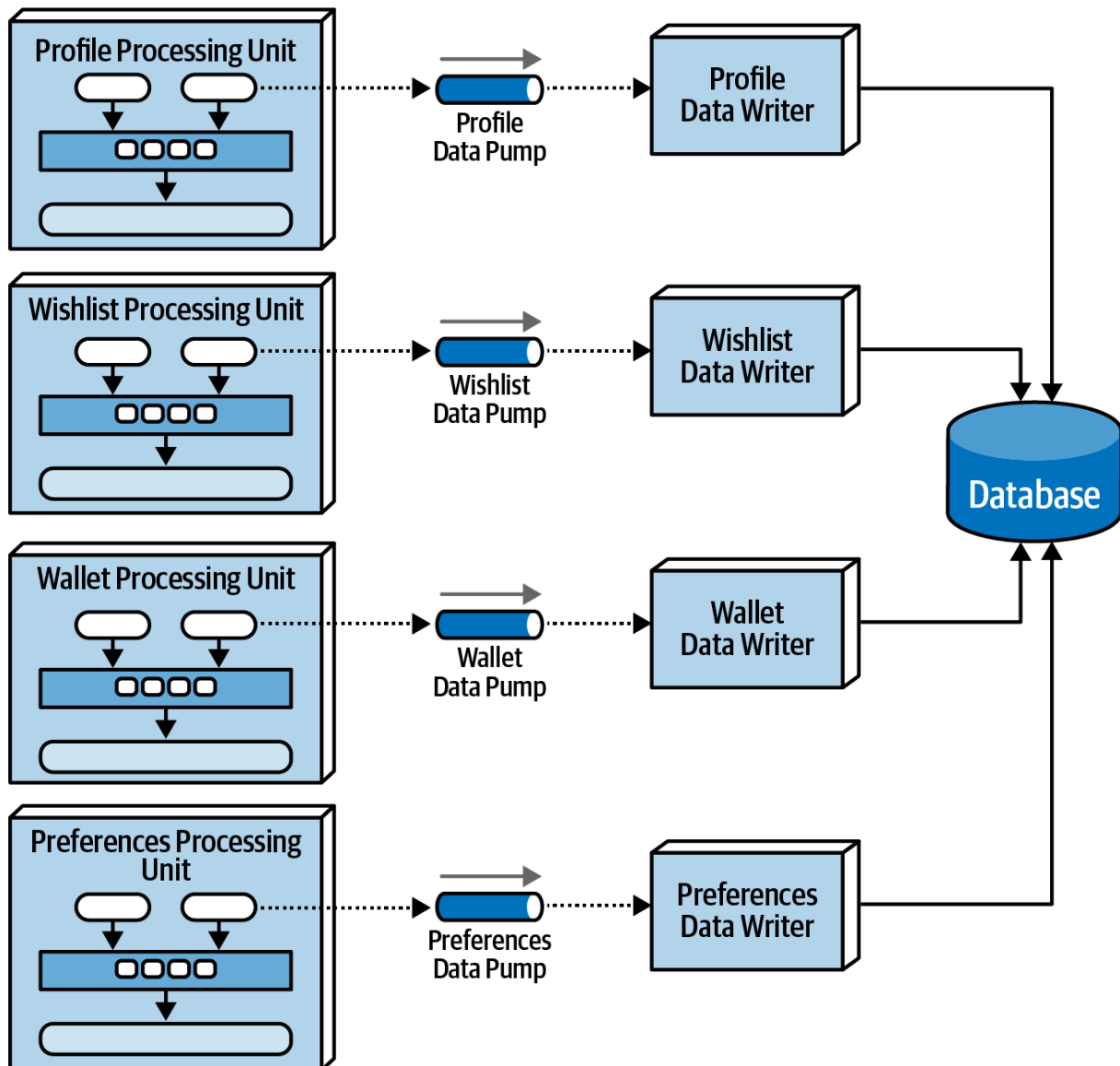
Figure 15-9. Dedicated data writers for each data pump
