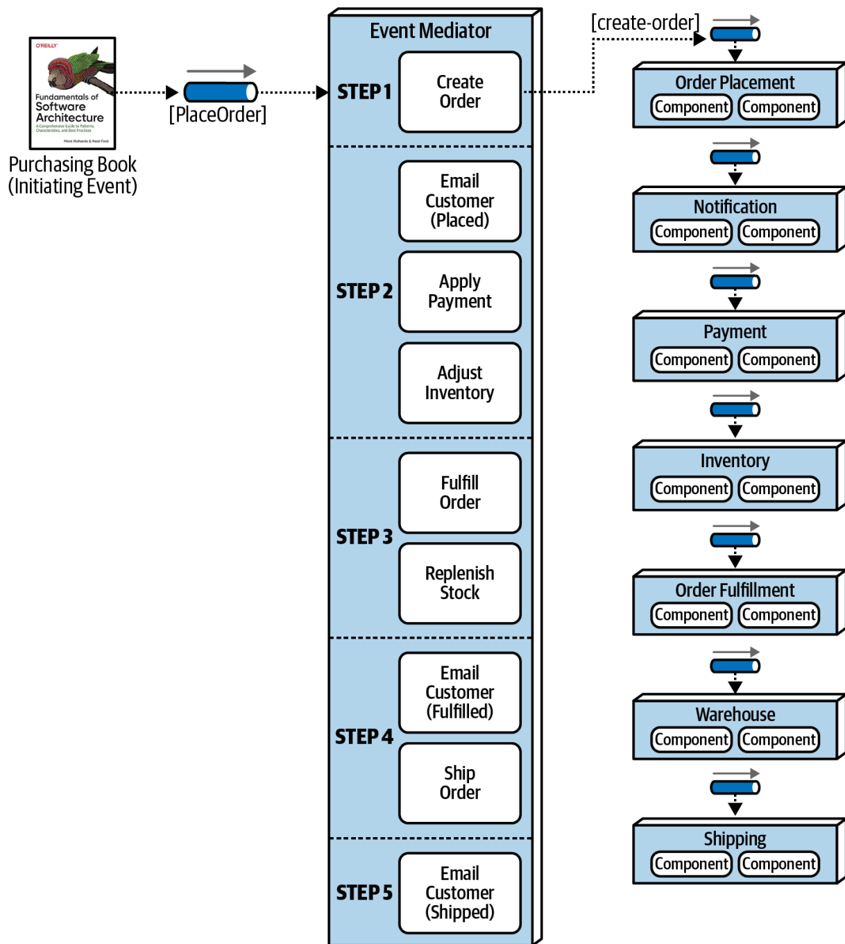
Figure 14-8. Step 1 of the mediator example
