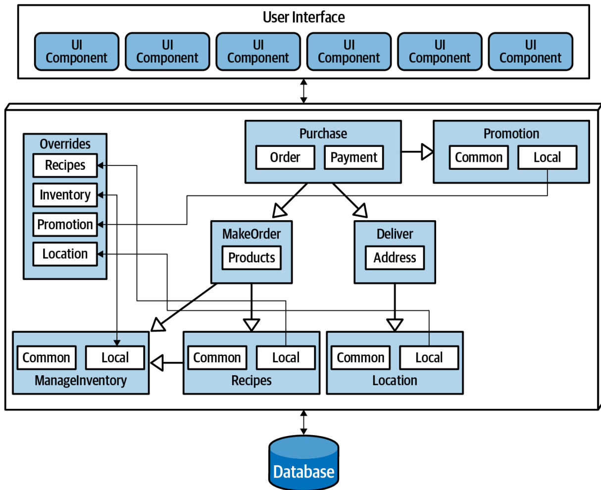
Figure 18-1. A modular monolith implementation of Silicon Sandwiches
