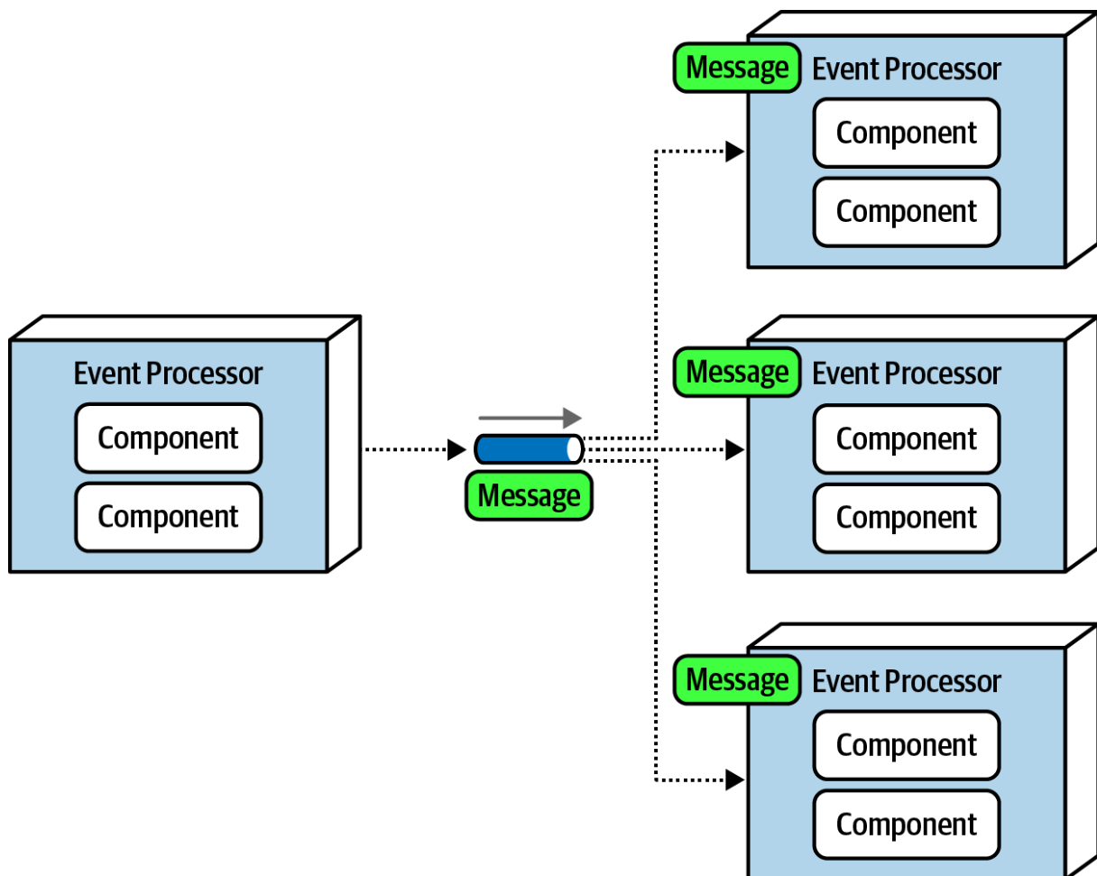
Figure 14-18. Broadcasting events to other event processors
