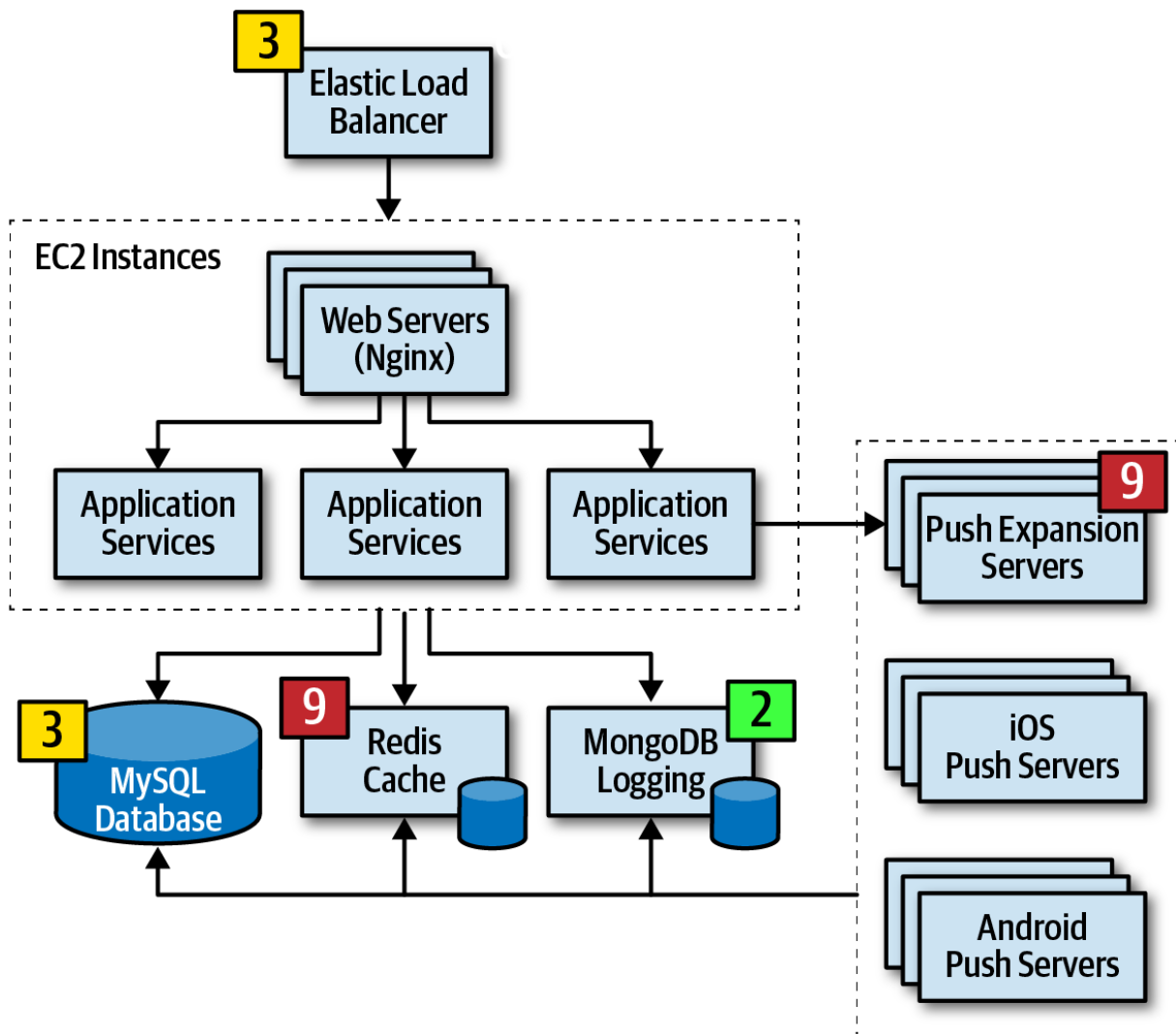
Figure 20-8. Consensus of risk areas
