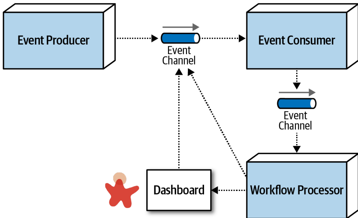
Figure 14-14. Workflow event pattern of reactive architecture
