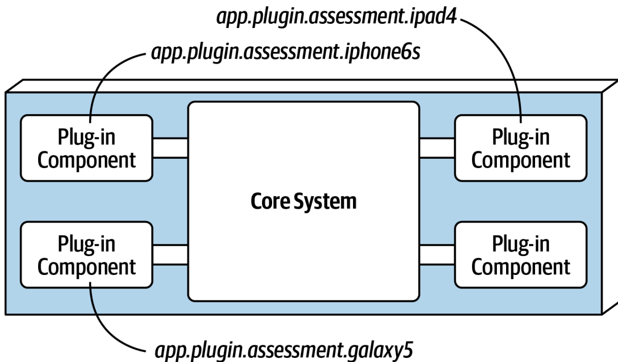
Figure 12-5. Package or namespace plug-in implementation
