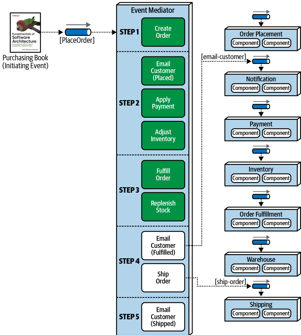
Figure 14-11. Step 4 of the mediator example
