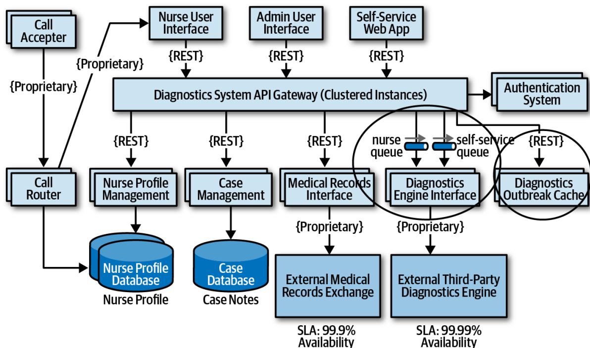
Figure 20-12. Architecture modifications to address elasticity risk
