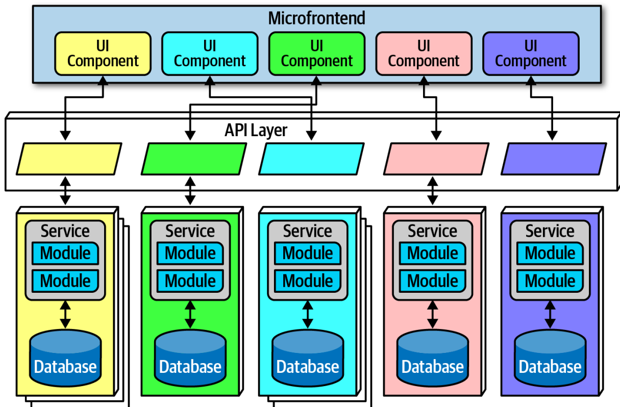
Figure 17-6. Microfrontend pattern in microservices
