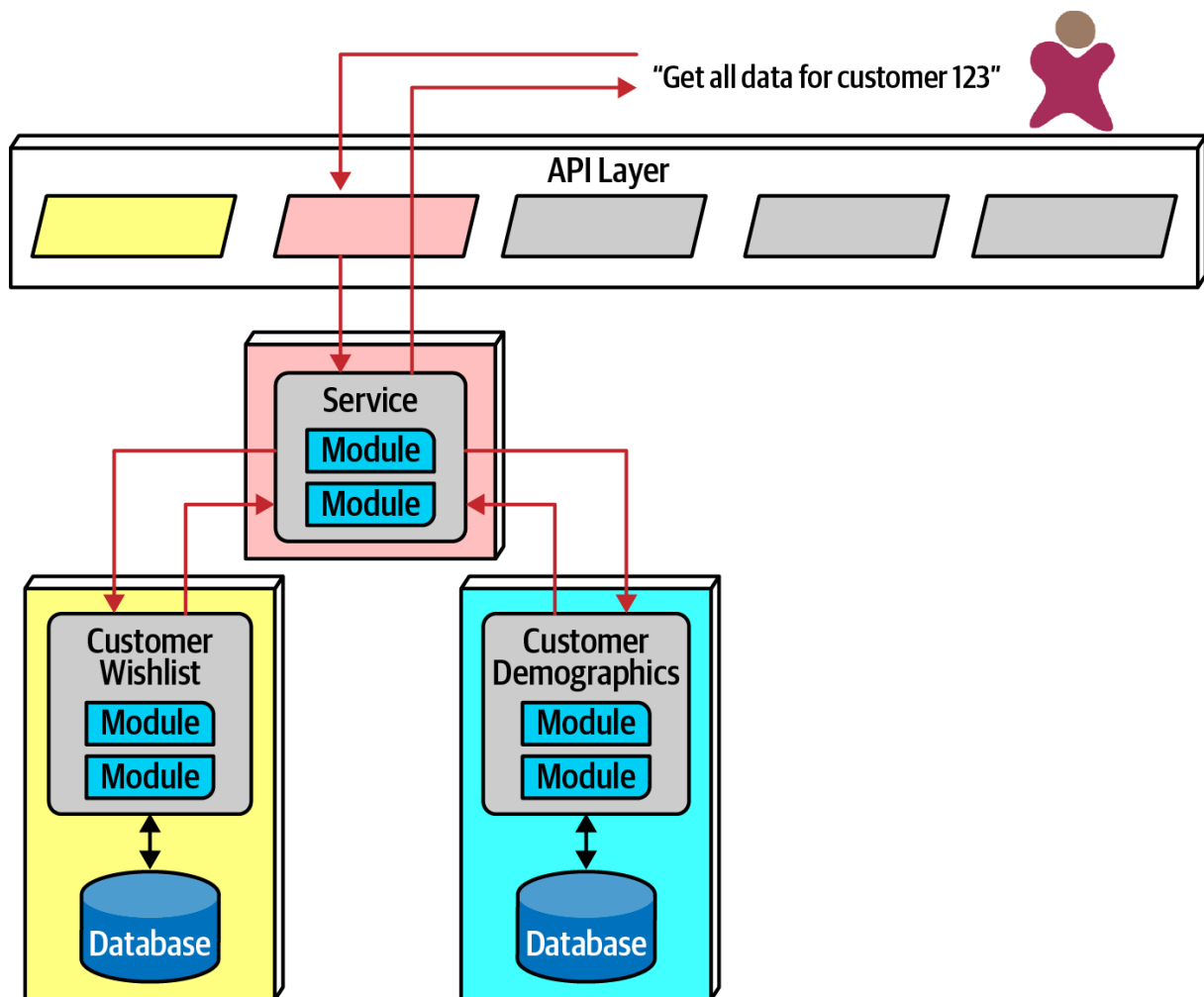
Figure 17-8. Using orchestration in microservices
