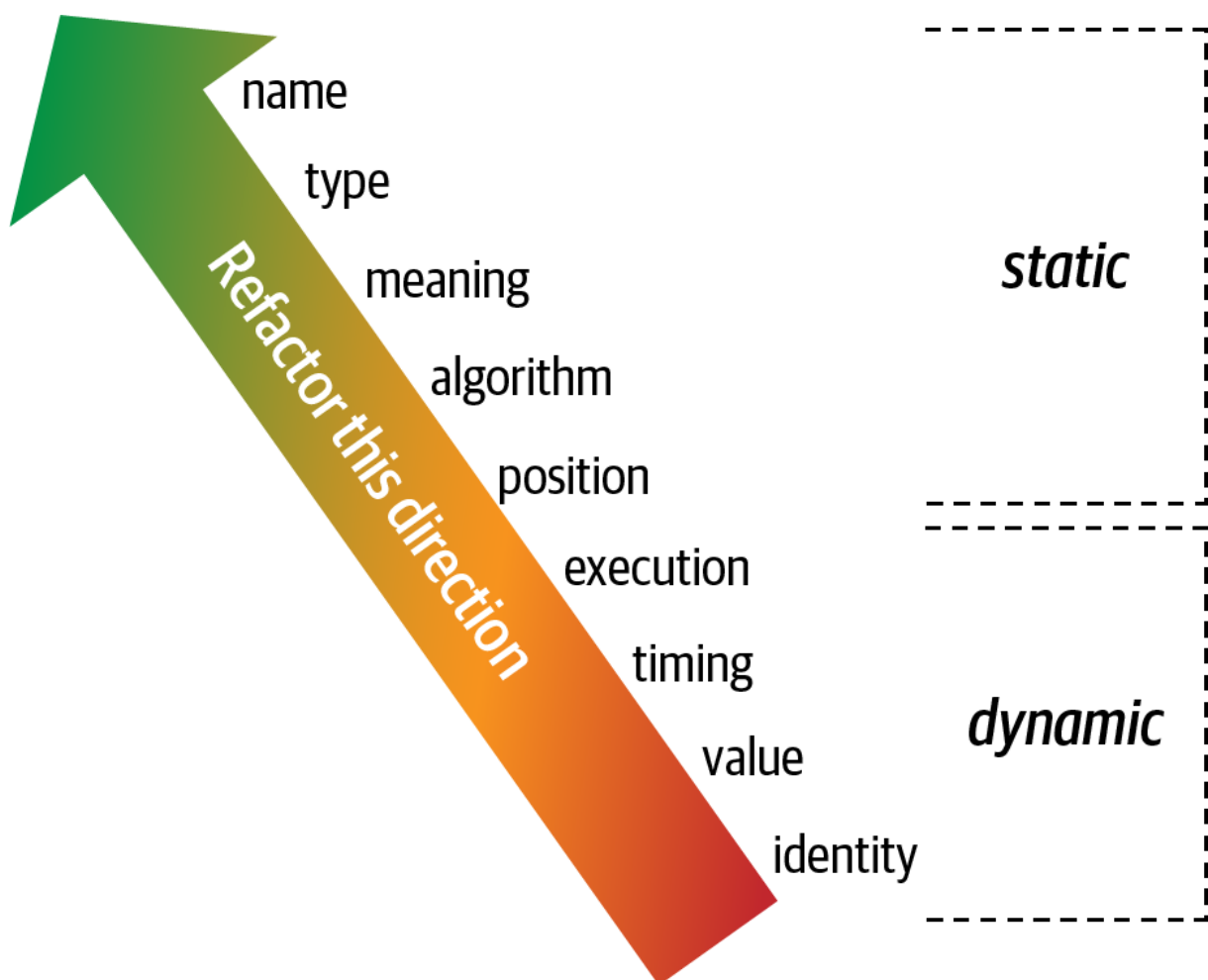
Figure 3-5. The strength on connascence provides a good refactoring guide
