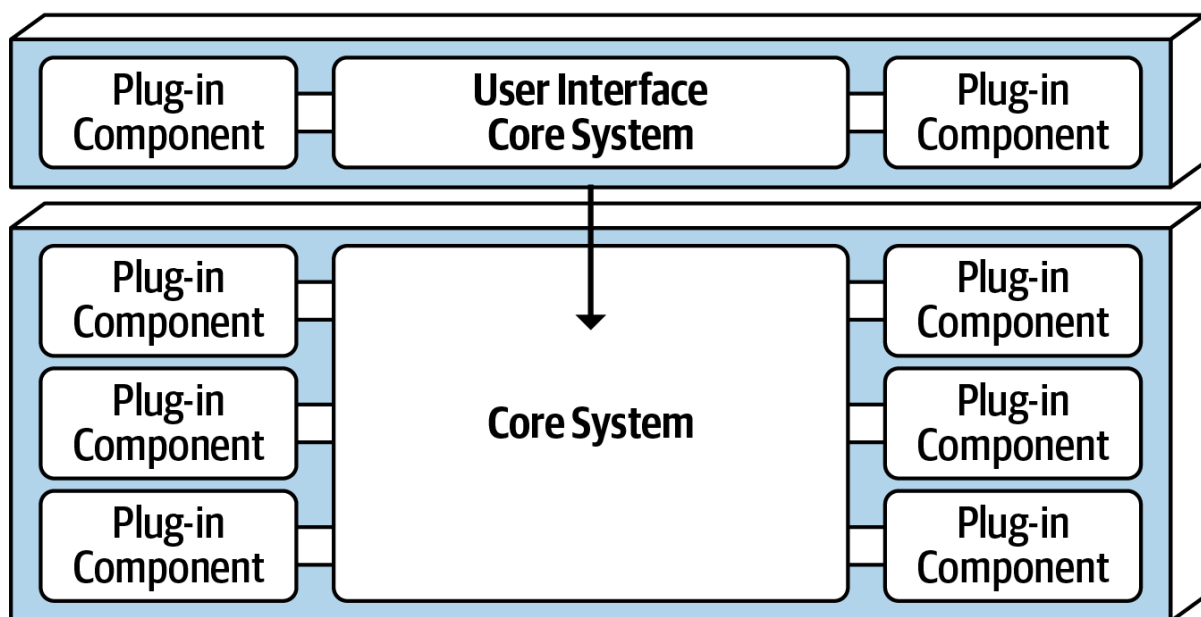
Separate User Interface (Multiple Deployment Units, Both Microkernel)
