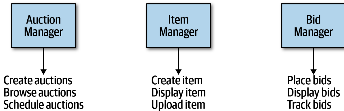
Figure 8-9. Building an architecture as an object-relational mapping
