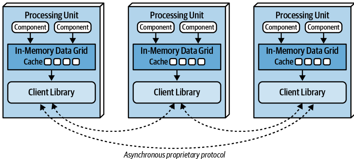
Figure 15-12. Replicated caching between processing units
