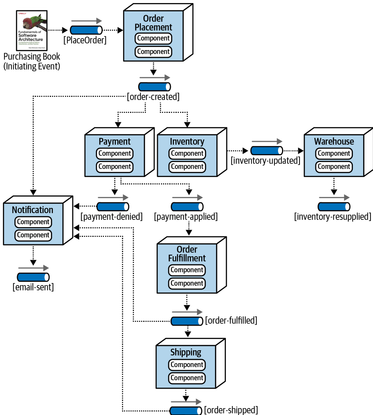
Figure 14-4. Example of the broker topology
