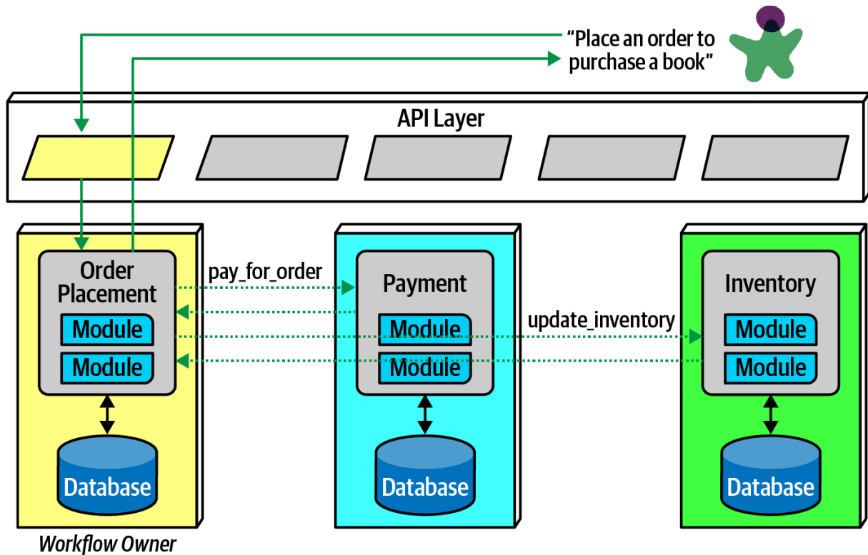
Figure 17-9. Using choreography for a complex business process
