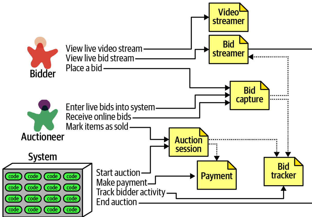
Figure 8-10. Initial set of components for Going, Going, Gone
