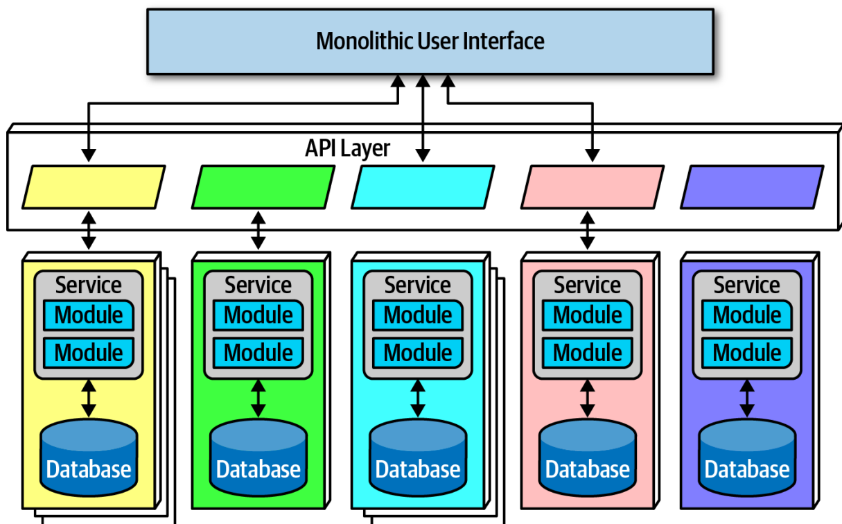
Figure 17-5. Microservices architecture with a monolithic user interface
