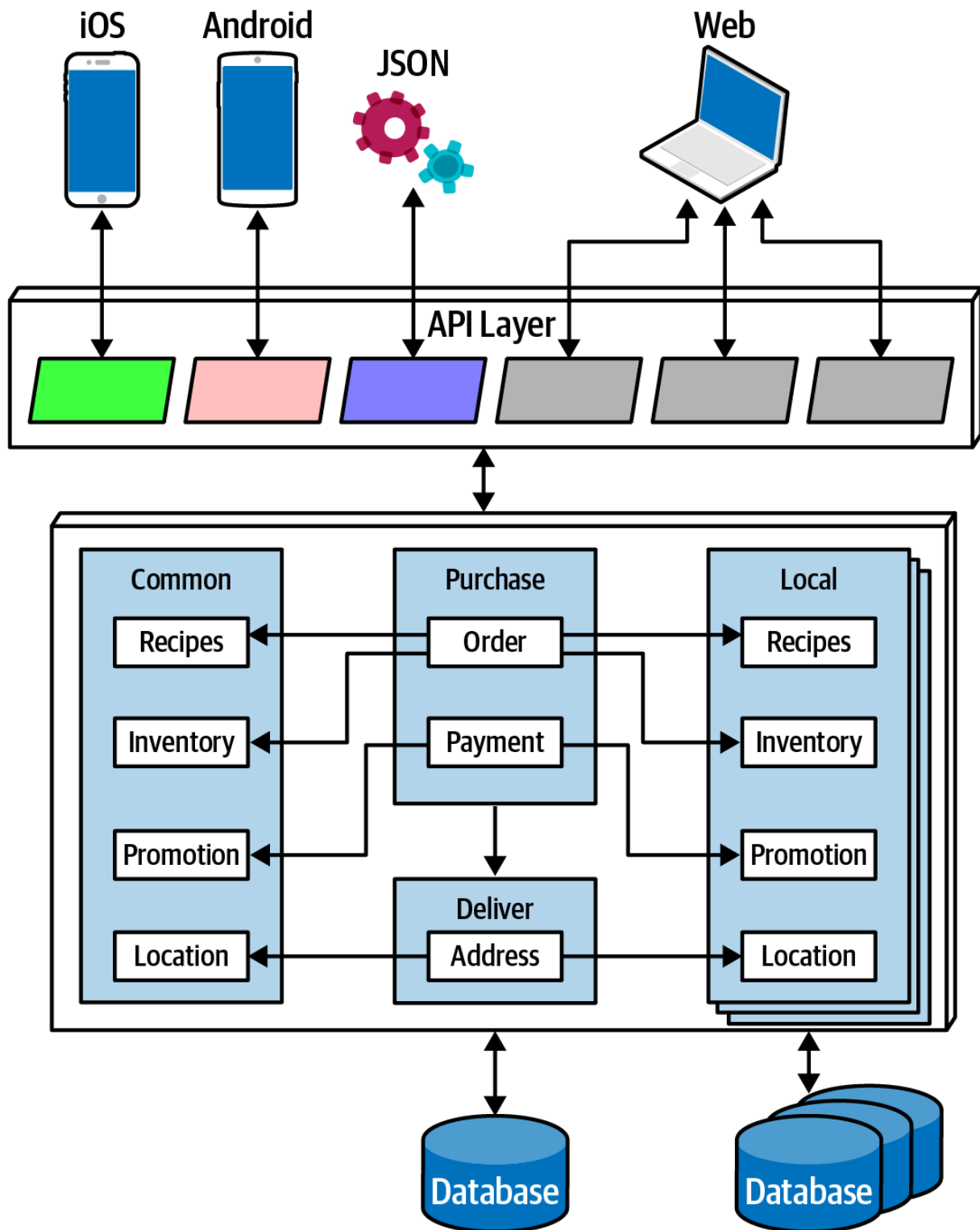
Figure 18-2. A microkernel implementation of Silicon Sandwiches
