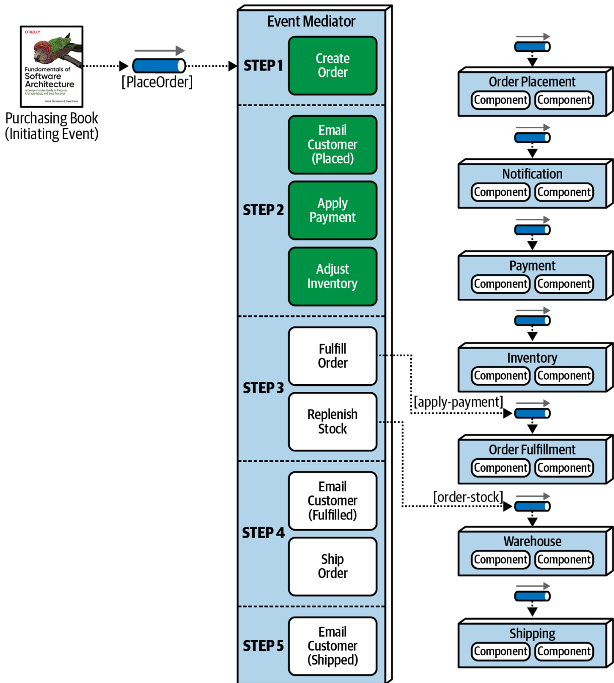
Figure 14-10. Step 3 of the mediator example
