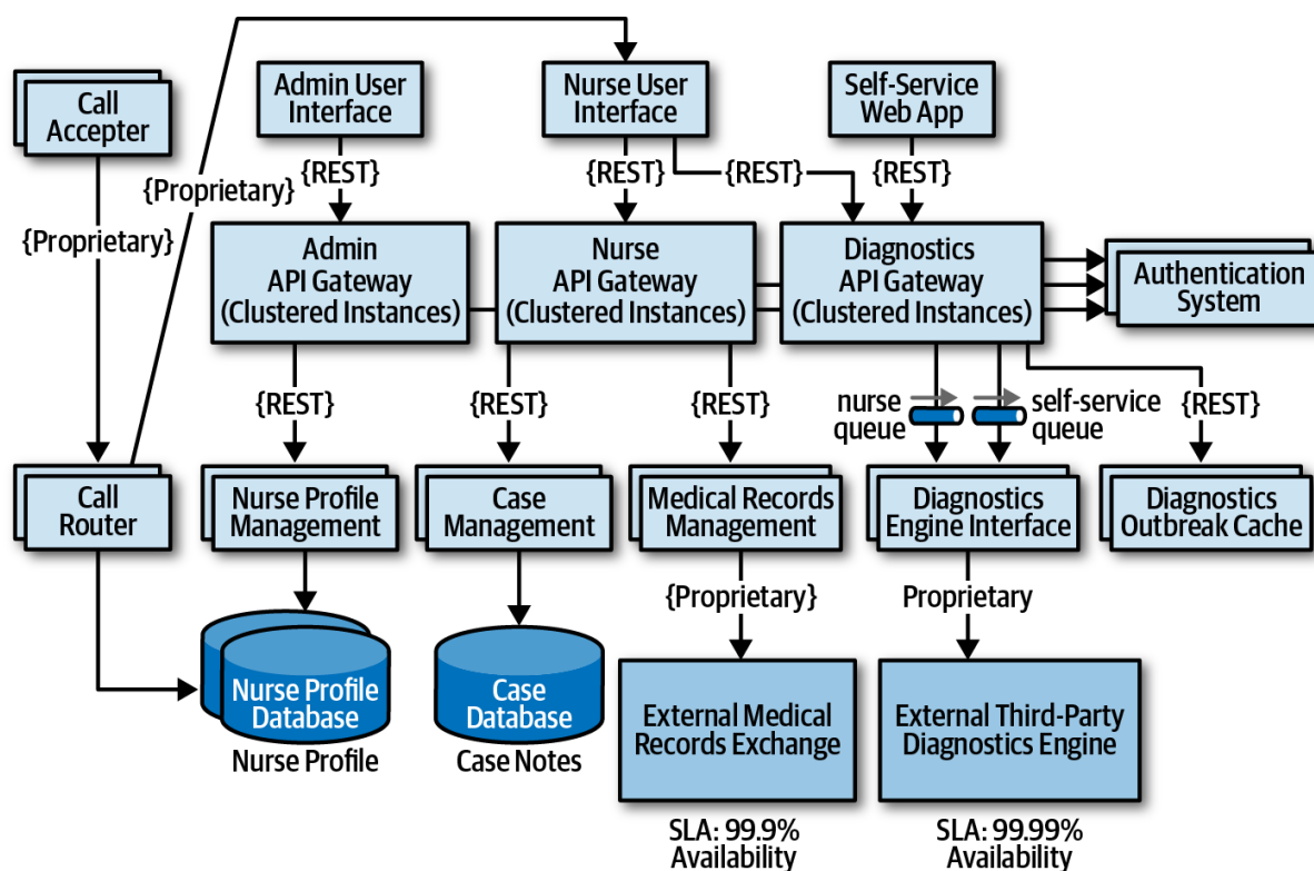
Figure 20-13. Final architecture modifications to address security risk
