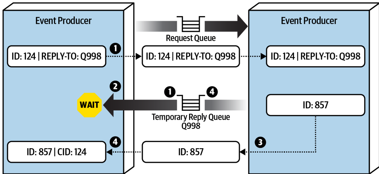
Figure 14-21. Request-reply message processing using a temporary queue
