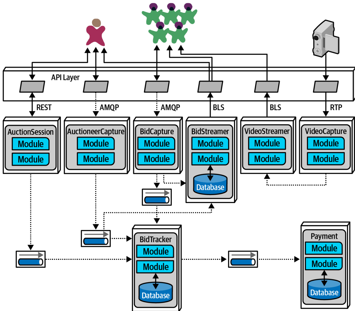
Figure 18-3. A microservices implementation of Going, Going, Gone
