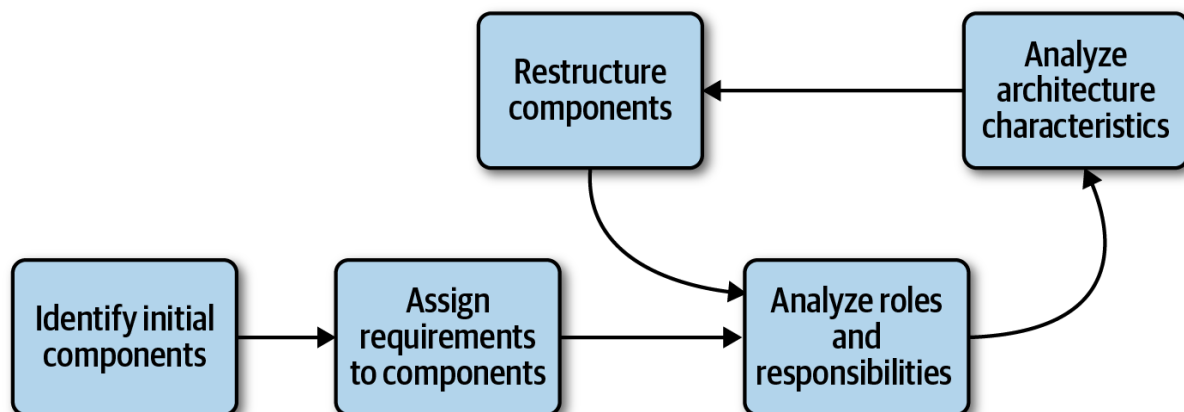
Figure 8-8. Component identification cycle
