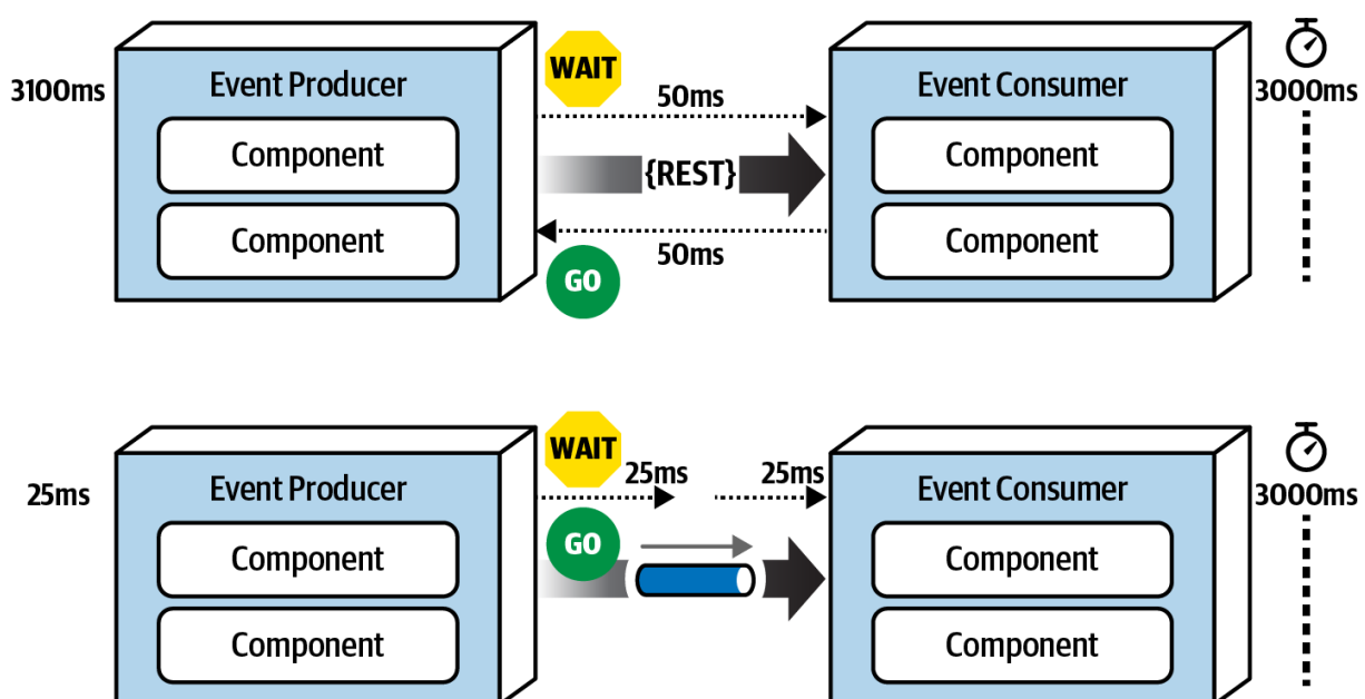
Figure 14-13. Synchronous versus asynchronous communication
