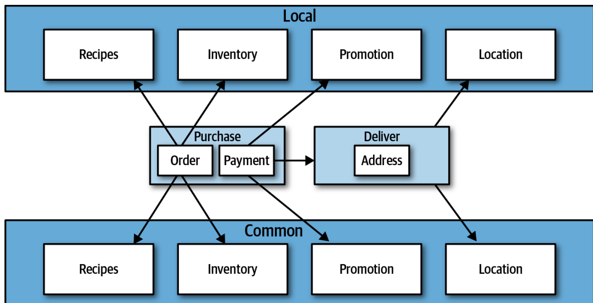
Figure 8-7. A technically partitioned design for Silicon Sandwiches
