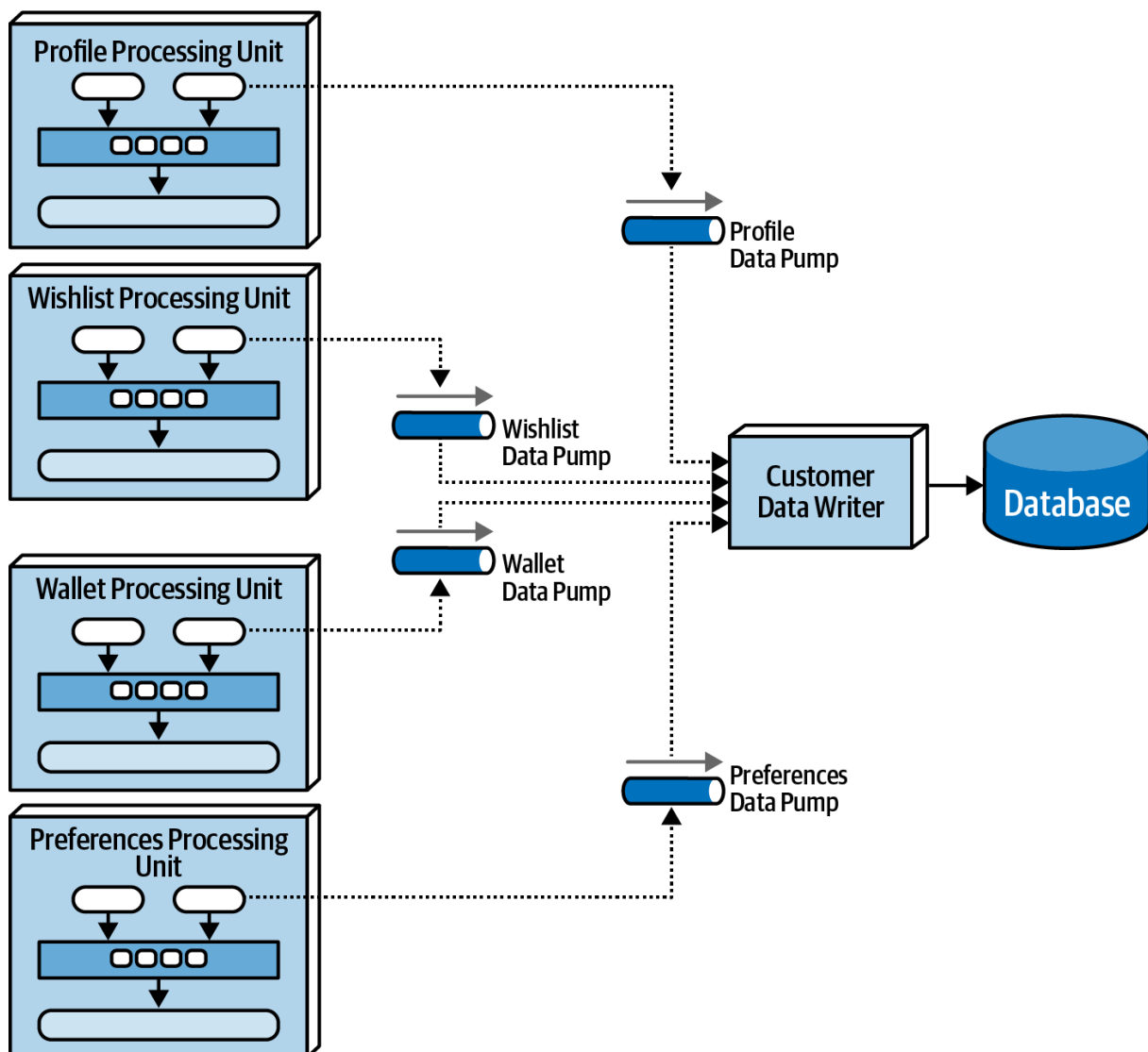
Figure 15-8. Domain-based data writer
