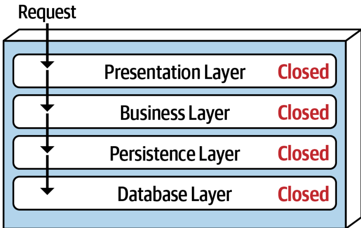
Figure 10-3. Closed layers within the layered architecture
