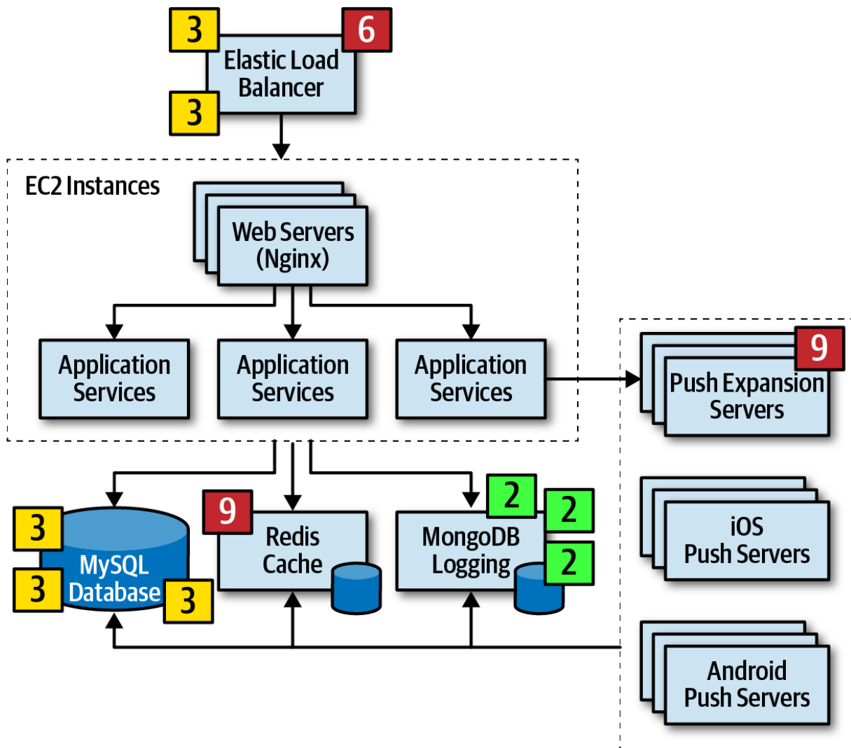
Figure 20-7. Initial identification of risk areas
