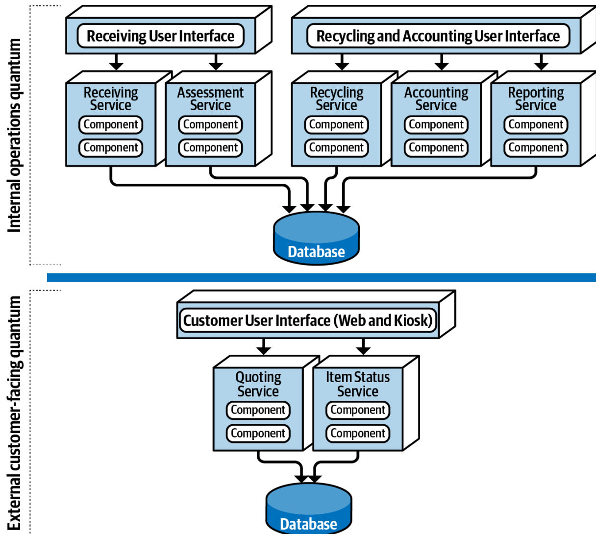
Figure 13-10. Separate quanta in a service-based architecture
