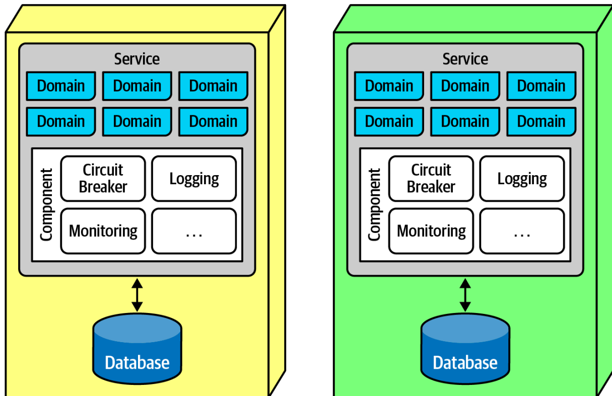
Figure 17-2. The sidecar pattern in microservices
