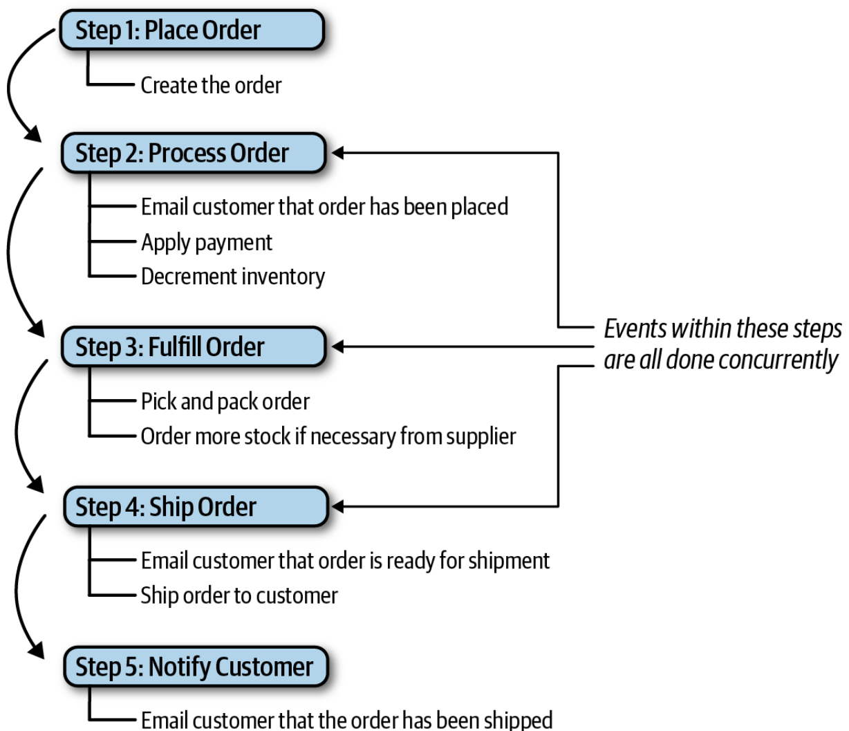
Figure 14-7. Mediator steps for placing an order
