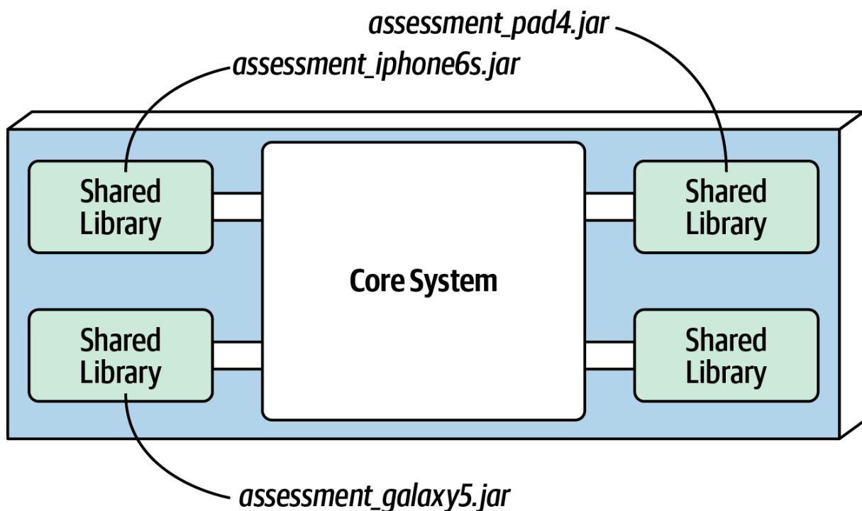
Figure 12-4. Shared library plug-in implementation
