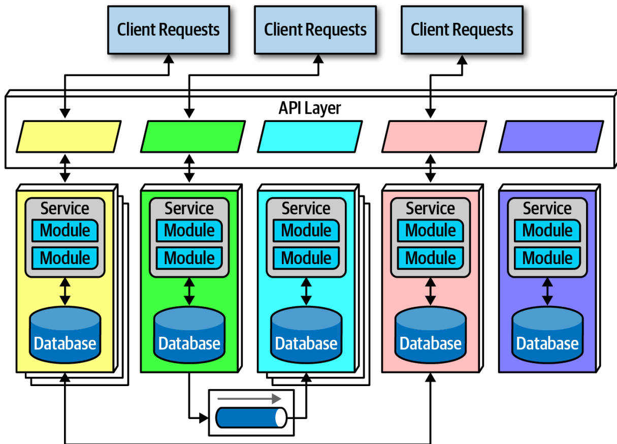
Figure 17-1. The topology of the microservices architecture style
