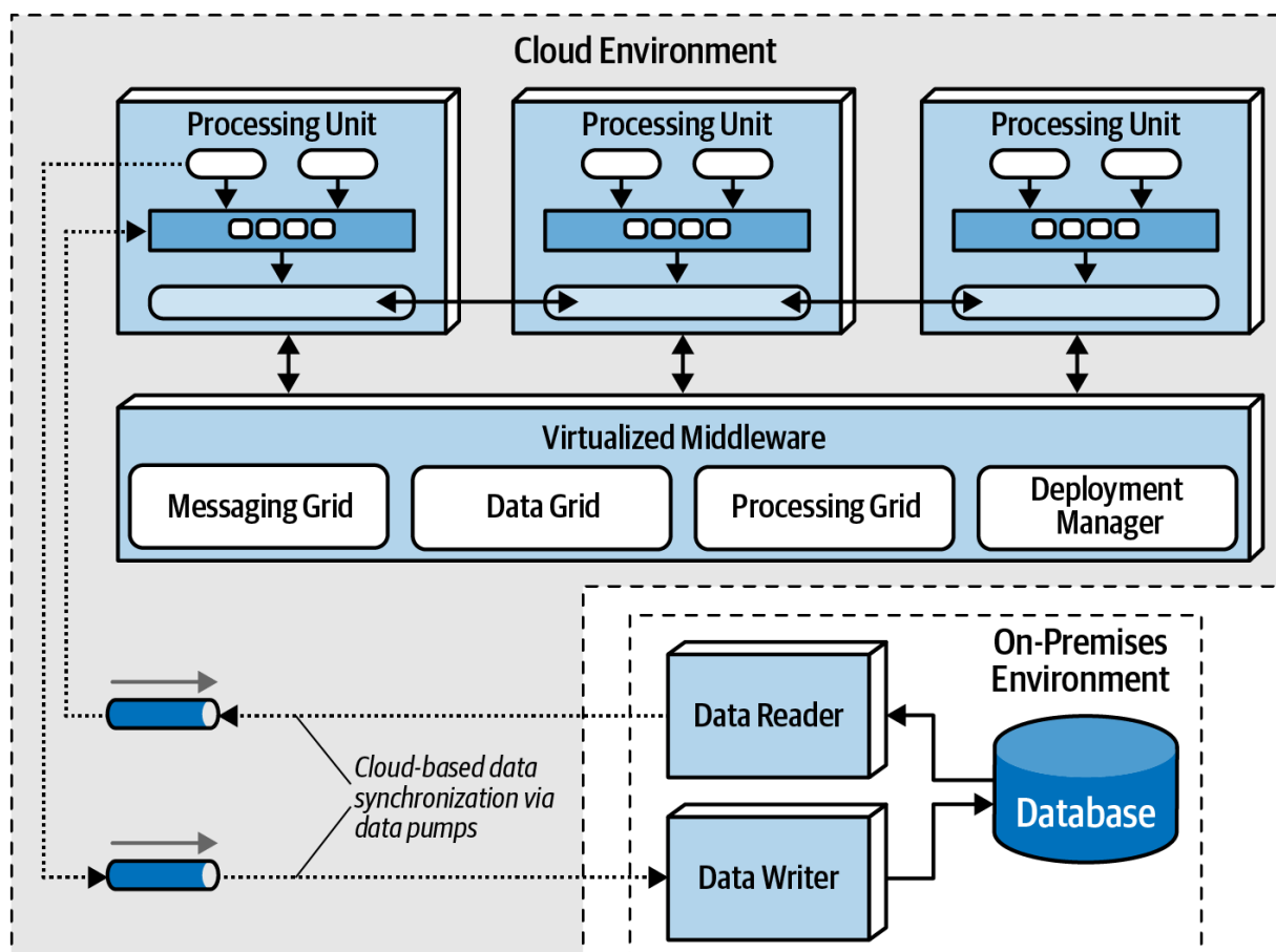
Figure 15-11. Hybrid cloud-based and on-prem topology
