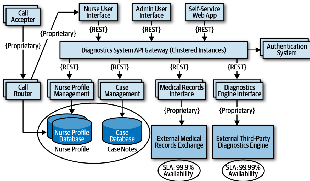
Figure 20-11. Architecture modifications to address availability risk
