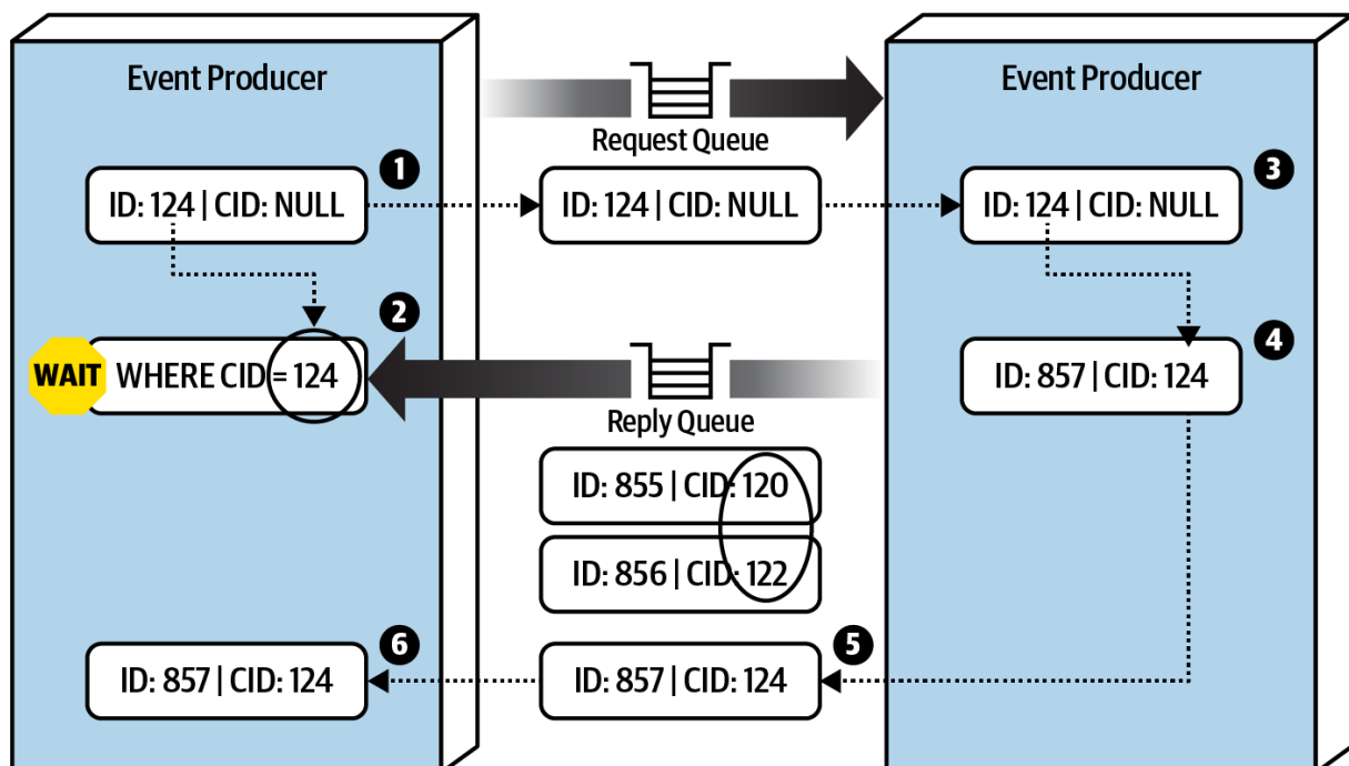
Figure 14-20. Request-reply message processing using a correlation ID
