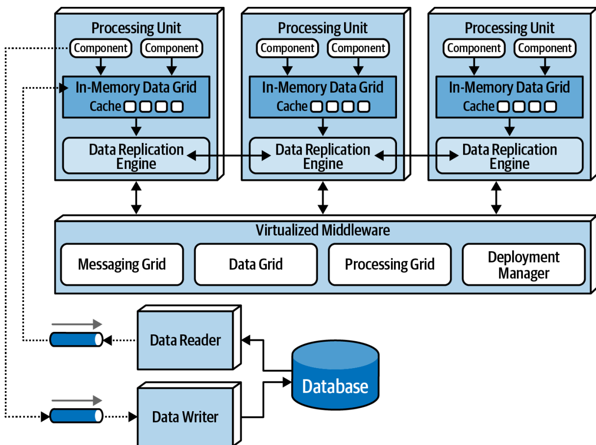
Figure 15-2. Space-based architecture basic topology
