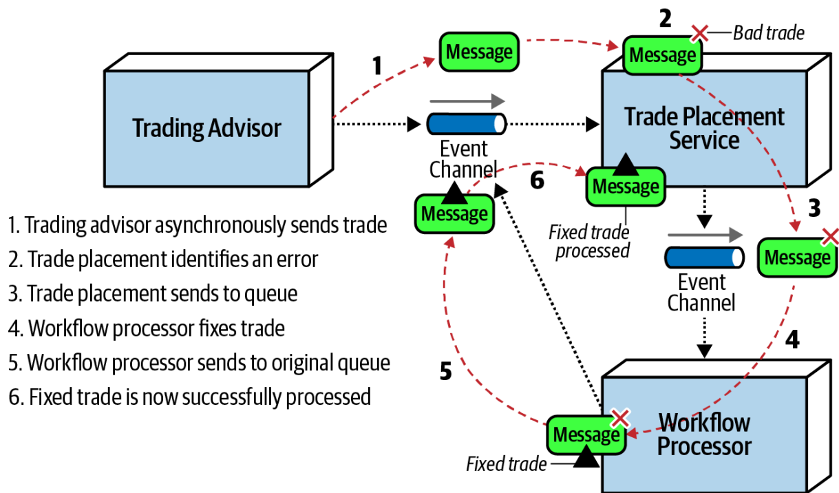
Figure 14-15. Error handling with the workflow event pattern
