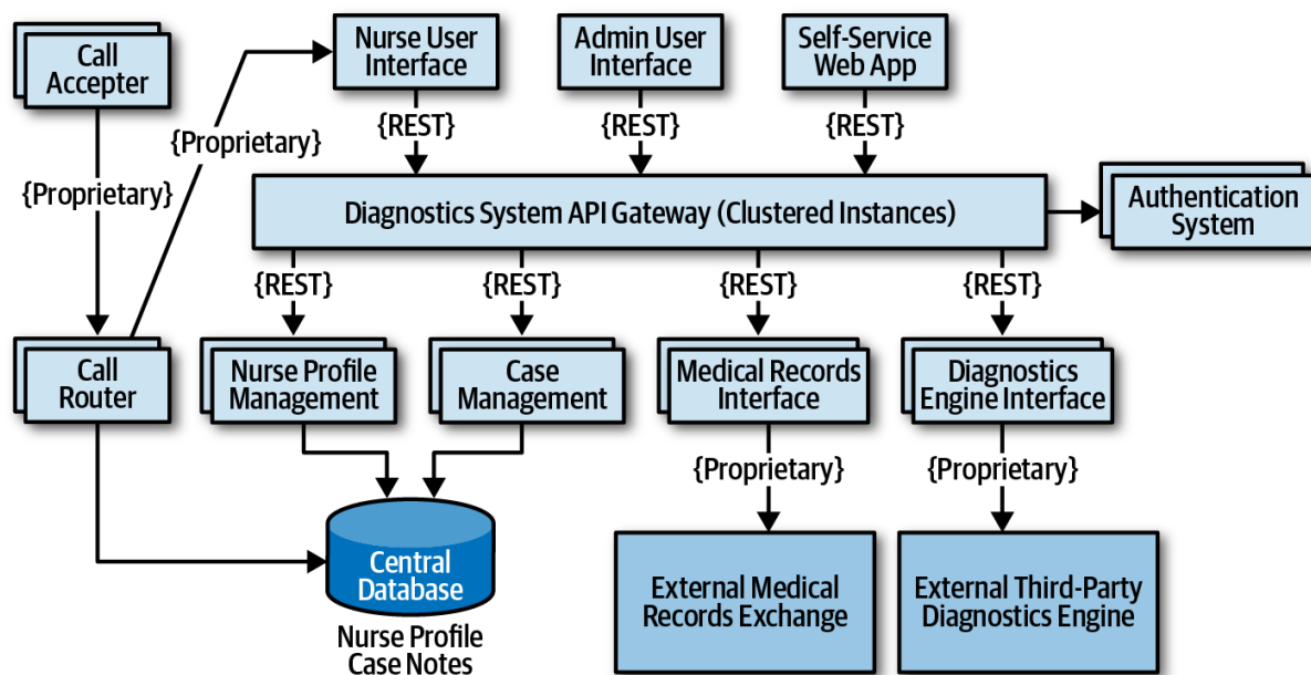
Figure 20-9. High-level architecture for nurse diagnostics system example
