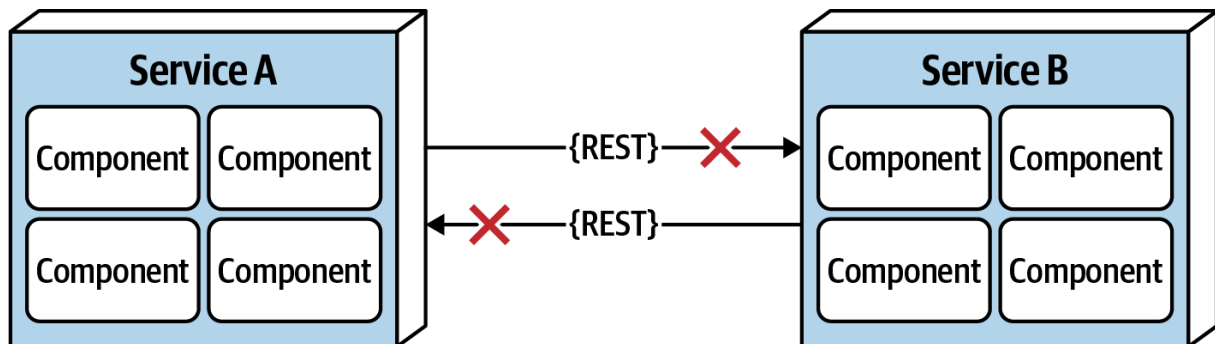
Figure 9-2. The network is not reliable
