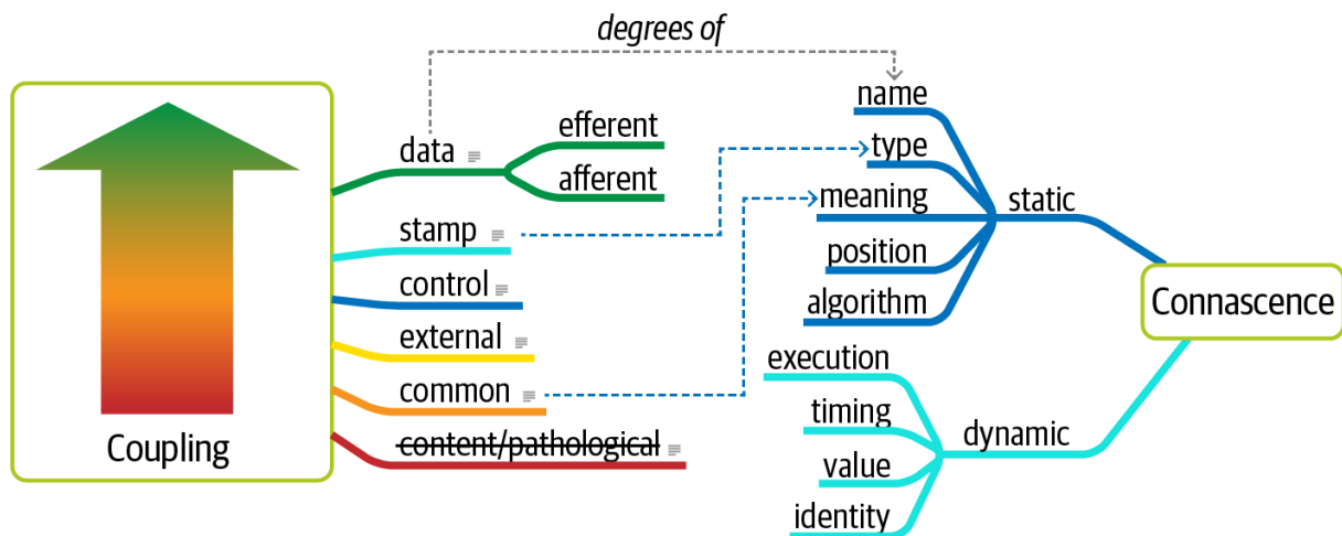
Figure 3-6. Unifying coupling and connascence
