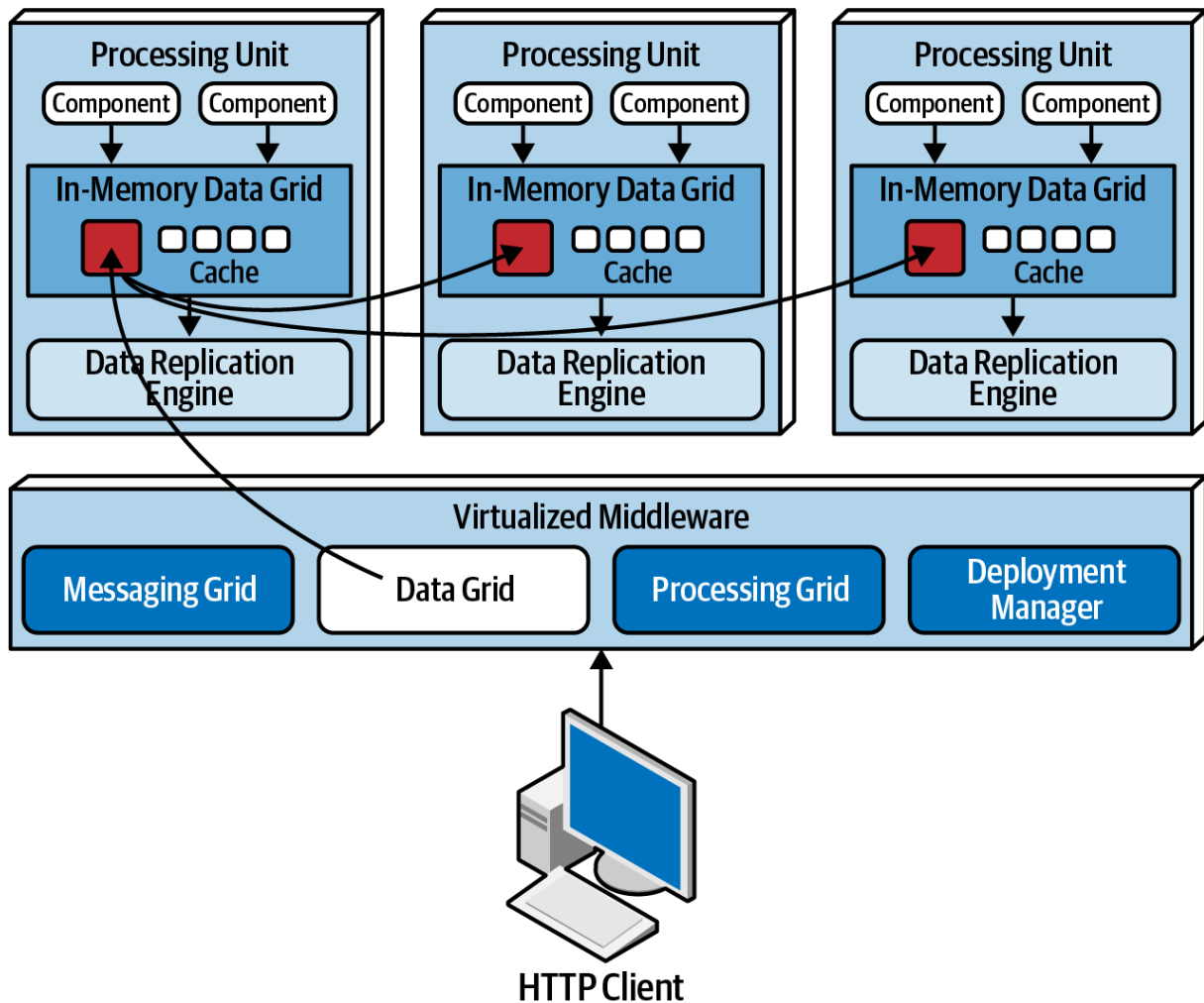
Figure 15-5. Data grid
