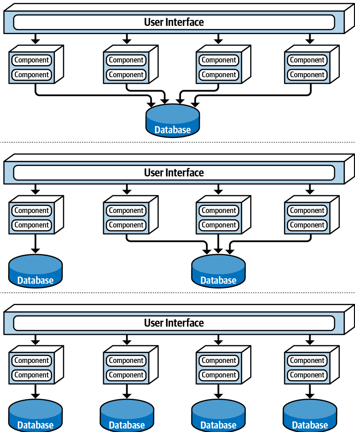
Figure 13-3. Database variants
