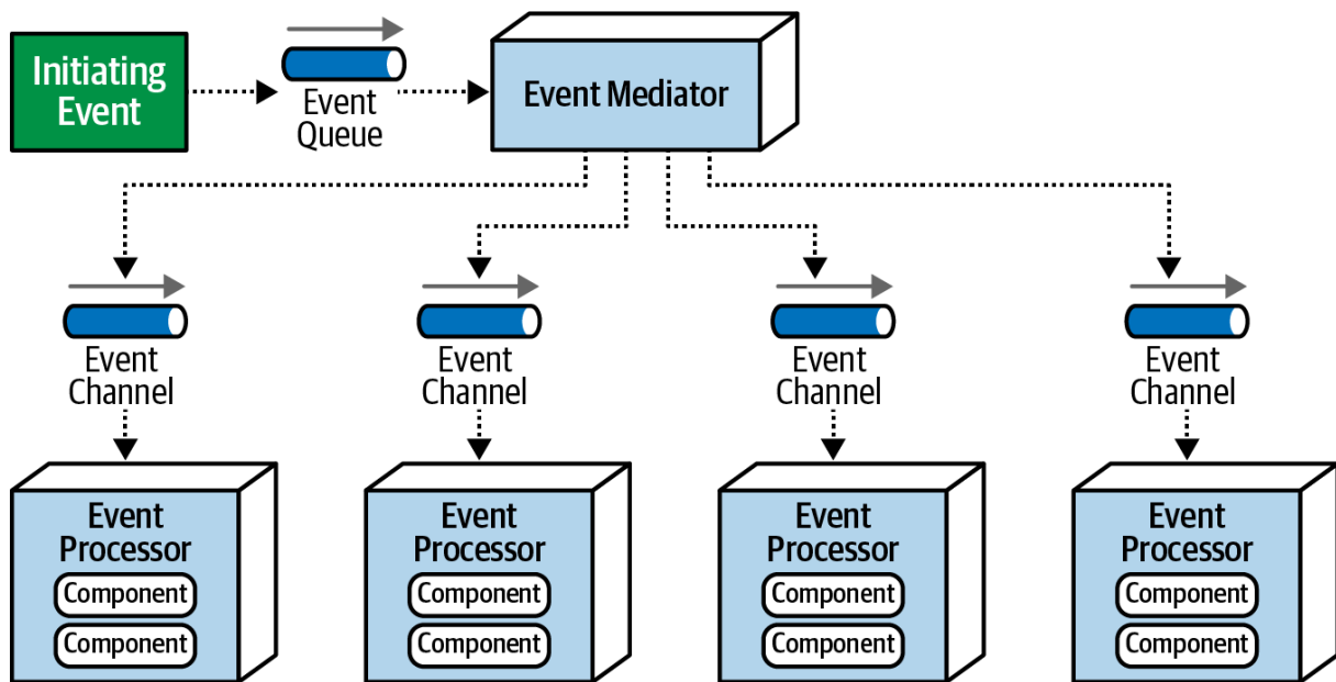
Figure 14-5. Mediator topology
