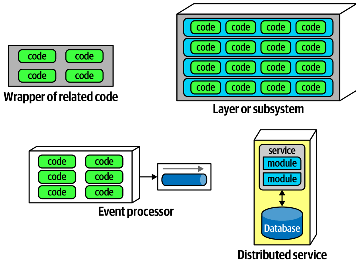
Figure 8-1. Different varieties of components
