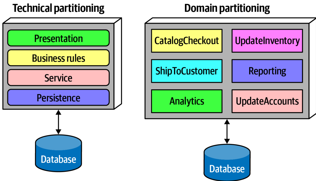
Figure 8-4. Two types of top-level partitioning in architecture
