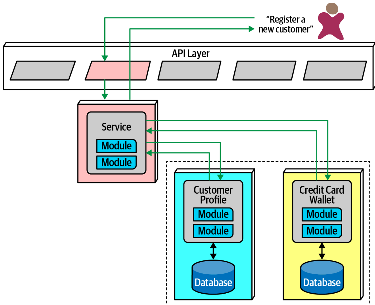
Figure 17-11. The saga pattern in microservices architecture
