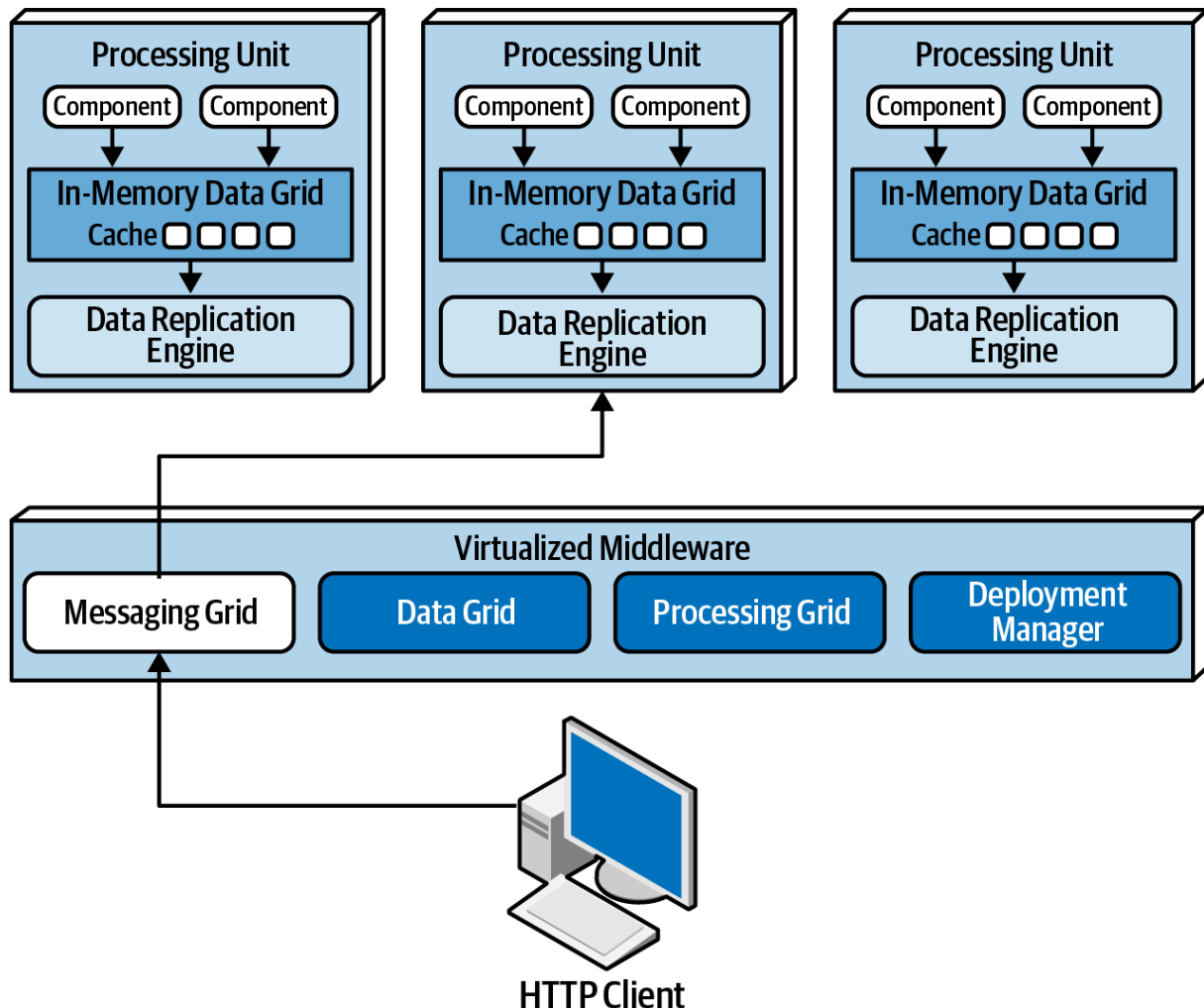
Figure 15-4. Messaging grid
