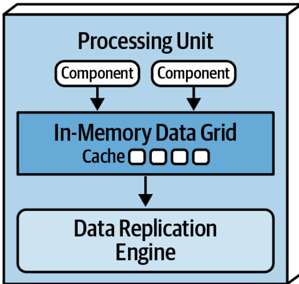
Figure 15-3. Processing unit
