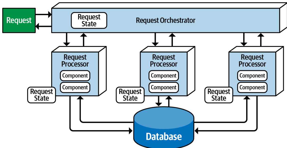
Figure 14-1. Request-based model
