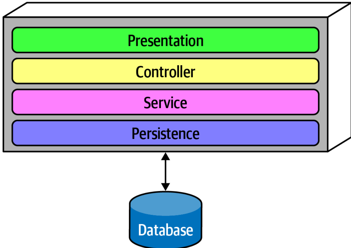
Figure 6-4. Layered architecture
