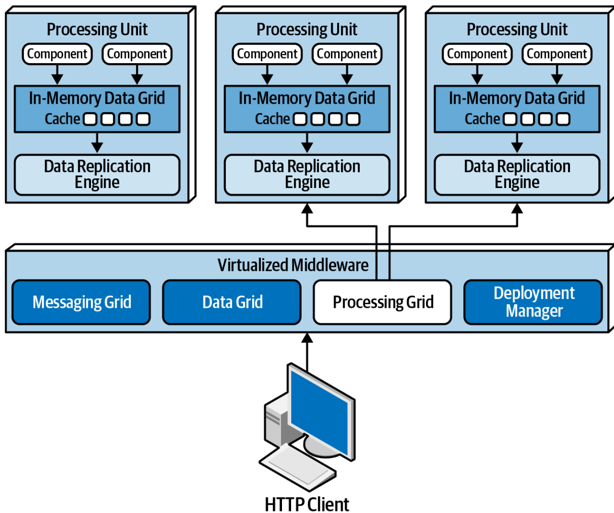
Figure 15-6. Processing grid
