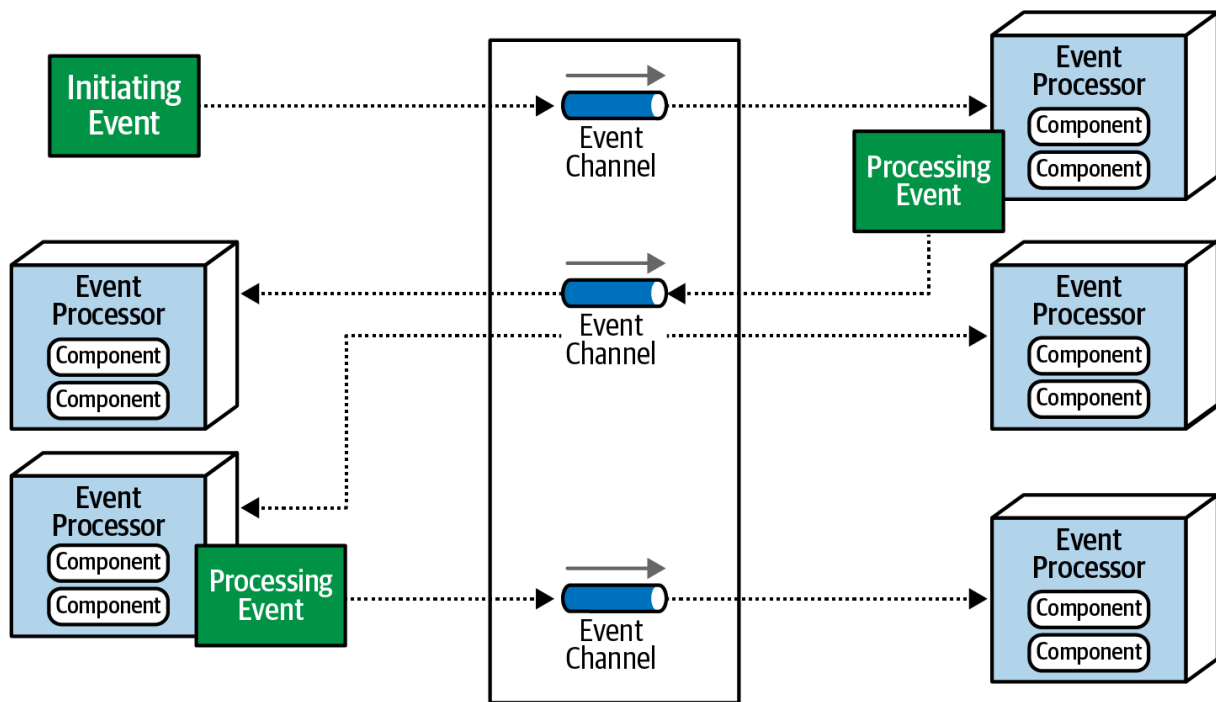
Figure 14-2. Broker topology
