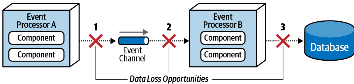
Figure 14-16. Where data loss can happen within an event-driven architecture
