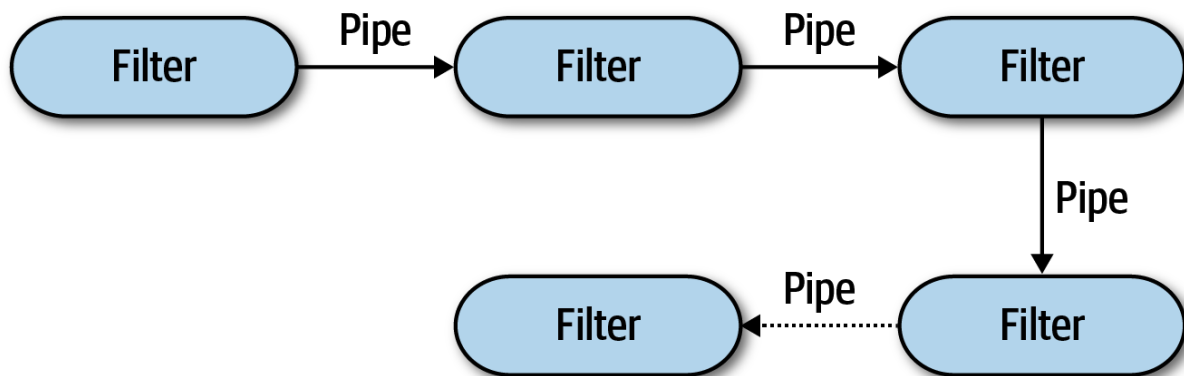
Figure 11-1. Basic topology for pipeline architecture
