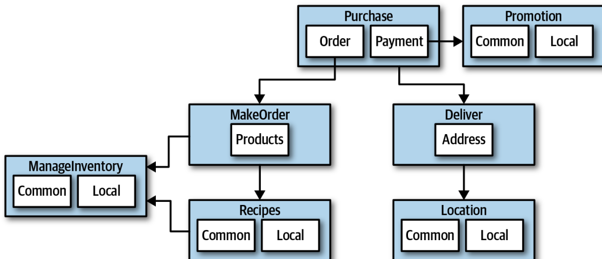
Figure 8-6. A domain-partitioned design for Silicon Sandwiches
