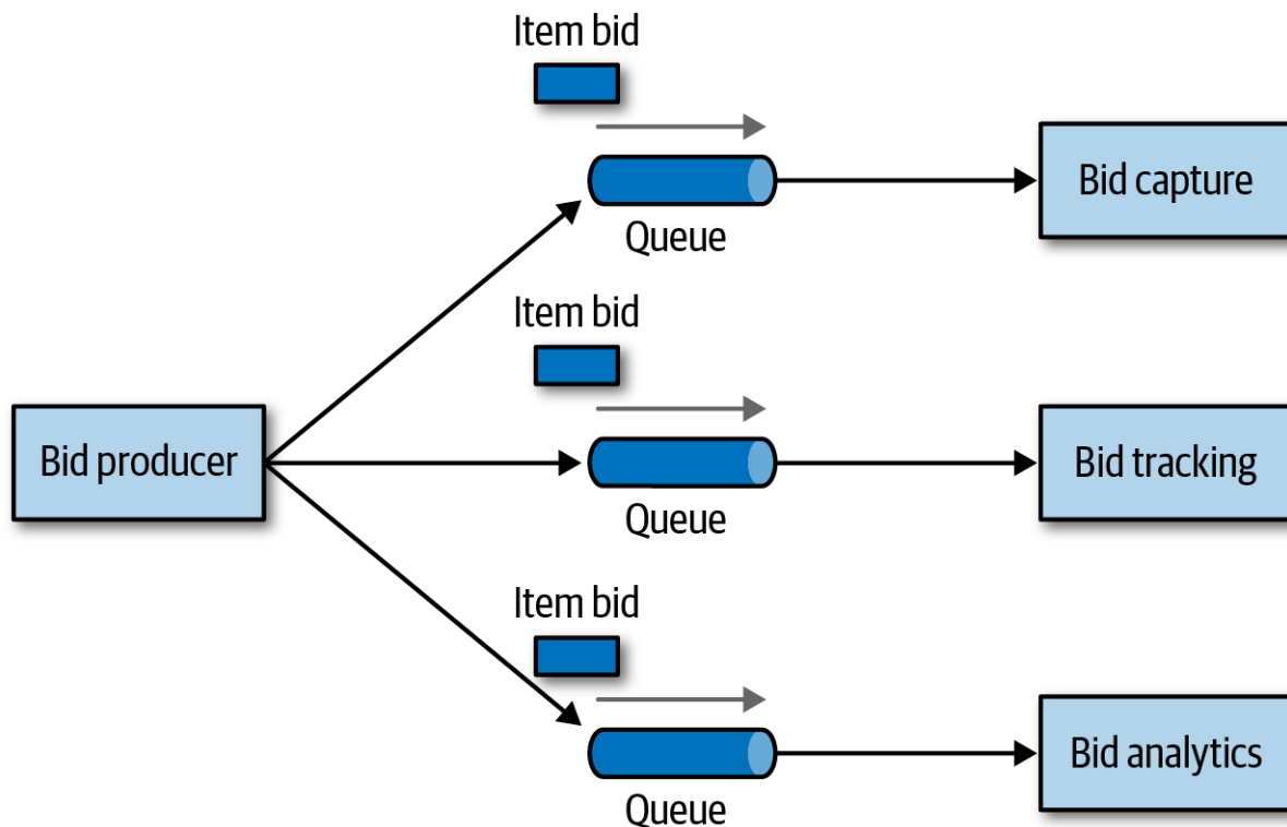
Figure 2-9. Use of queues for communication between services
