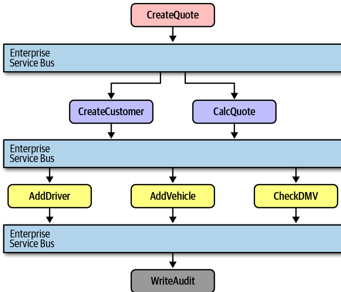
Figure 16-2. Message flow with service-oriented architecture
