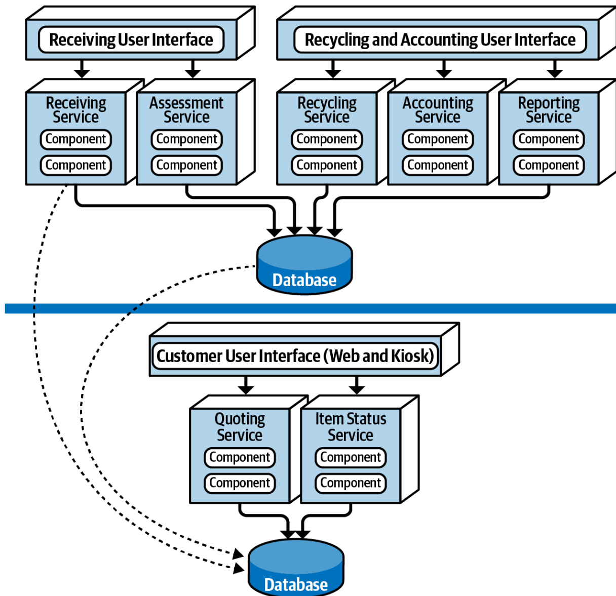
Figure 13-8. Electronics recycling example using service-based architecture
